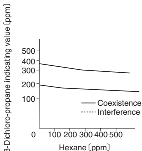
FIG. 1 Influence of Hexane
