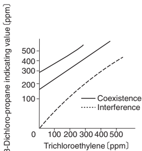
FIG. 2 Influence of Trichloroethylene
